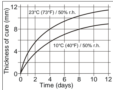
Diagram 1: Curing speed of Sikaflex®-529 AT
